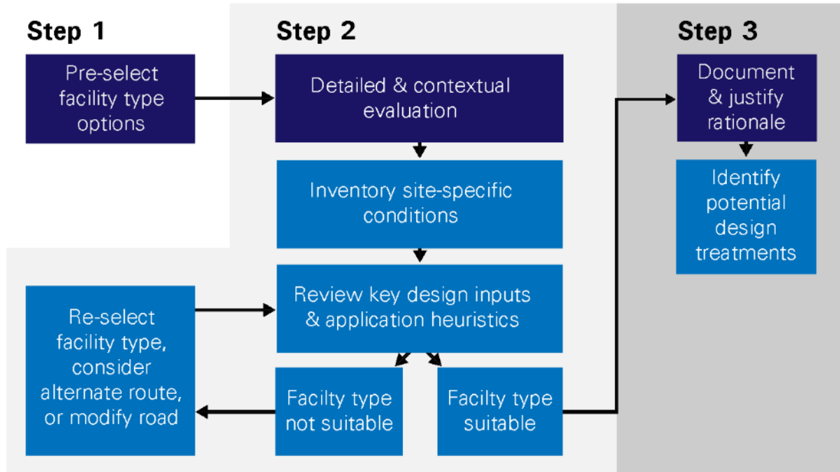
Figure 5-5: Three Step Facility Selection Flow Chart (Source: OTM Book 18)
